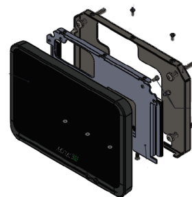
Fixed Wall Mechanical Support (Ref. PRD10706) *
