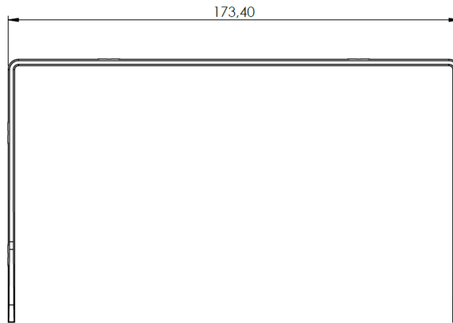
Side View Sunshade Support
