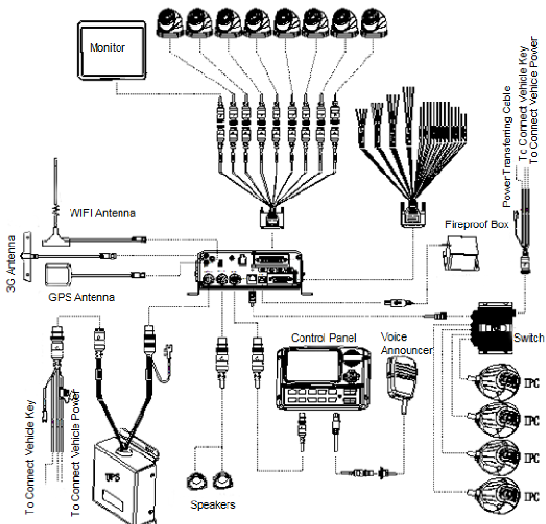
Diagram1 (POE Switch RJ45)
